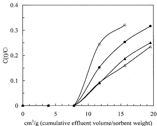
Figure 10. Breakthrough of benzothiophene (○) or dibenzothiophene (●) or 4-methyl-dibenzothiophene (△), or 4,6-dimethyl-dibenzothiophene (▲) in a fixed-bed adsorber with CuCl/γ-Al 2 O 3 adsorbent, with diesel feed at room-temperature.
