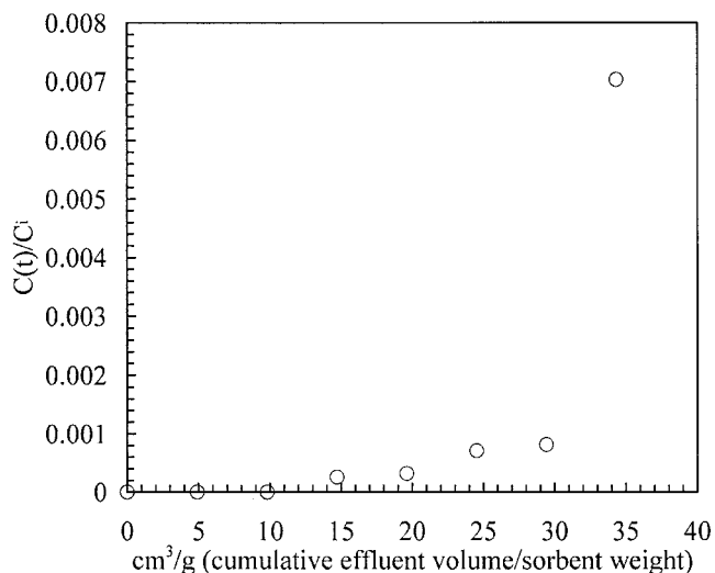
Figure 13. Breakthrough of total sulfur in a fixed-bed adsorber with AC/Cu(I)-Y adsorbents, for diesel feed at room-temperature.
