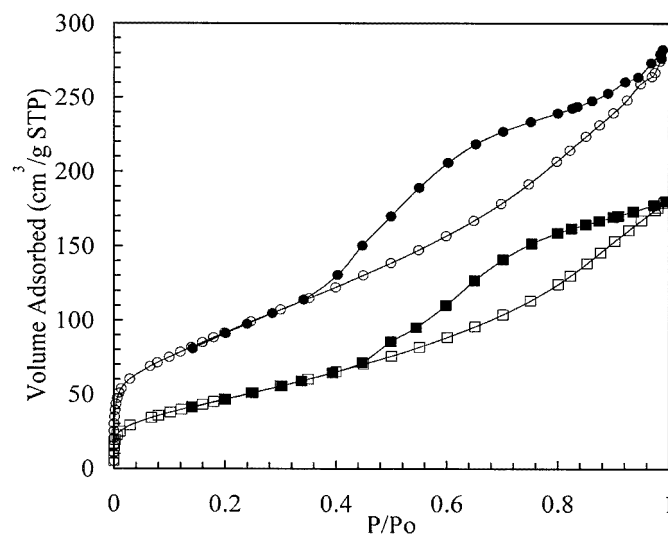
Figure 9. Equilibrium adsorption/desorption isotherms for nitrogen at -196°C on \gamma -Al 2 O 3 (○) and CuCl 2 / \gamma -Al 2 O 3 (□).
