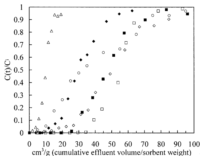
Figure 3. Breakthrough of total sulfur, for diesel feed at room-temperature, in a fixed-bed adsorber with: Cu(I)-ZSM-5 ( \Delta ), activated carbon ( \circ ), CuCl/ \gamma -Al 2 O 3 ( \blacklozenge ), Selexsorb® CDX alumina ( \diamond ), Cu(I)-Y ( \blacksquare ), and AC/Cu(I)-Y ( \square ).
