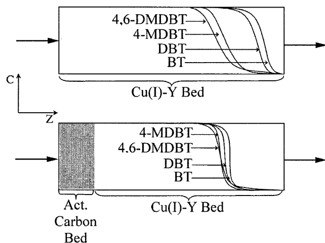
Figure 8. Concentration wavefronts of 4 sulfur compounds in adsorbents of Cu(I)Y and Cu(I)Y layered with 15% activated carbon, with diesel feed.
