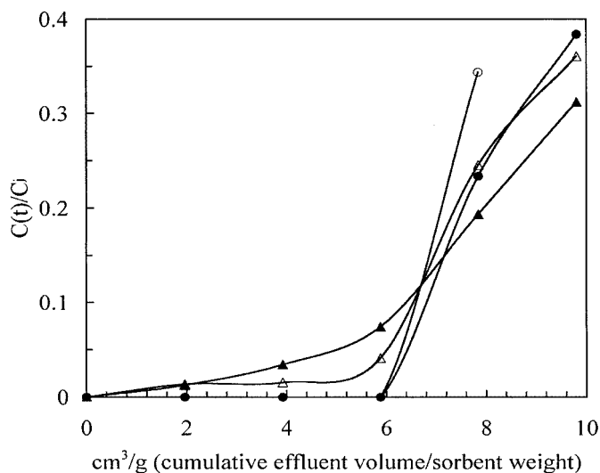
Figure 12. Breakthrough of benzothiophene (○) or dibenzothiophene (●) or 4-methyl-dibenzothiophene (△), or 4,6-dimethyl-dibenzothiophene (▲) in a fixed-bed adsorber with Cu(I)-ZSM-5 adsorbent, with diesel feed at room-temperature.
